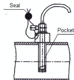
Fig. 11. Sealing of the PL type temperature probes
