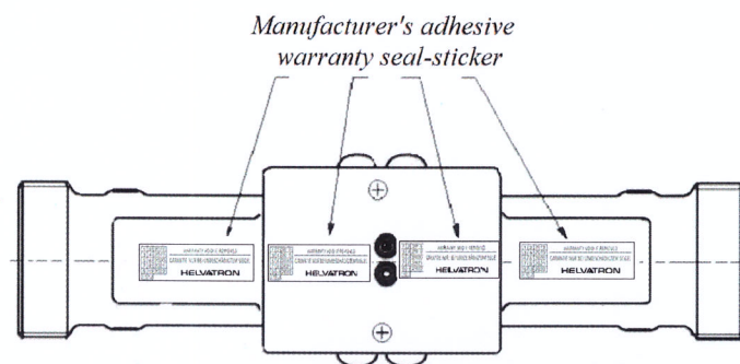
Fig. 9. Sealing of flow sensor q_p = 10/15/25/40/60 \text{ m}^3/\text{h}
