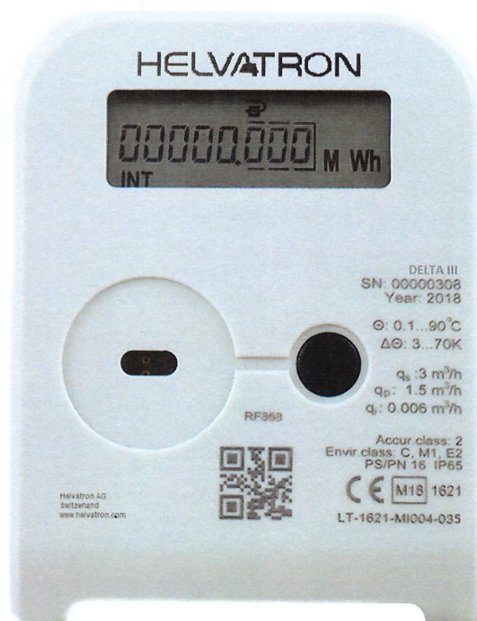
Fig.2. Calculator of the heat meter DELTA III
