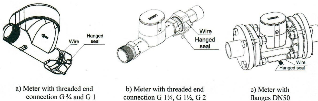
Fig.6. Sealing of the water meter QALCSONIC W1 after installation
