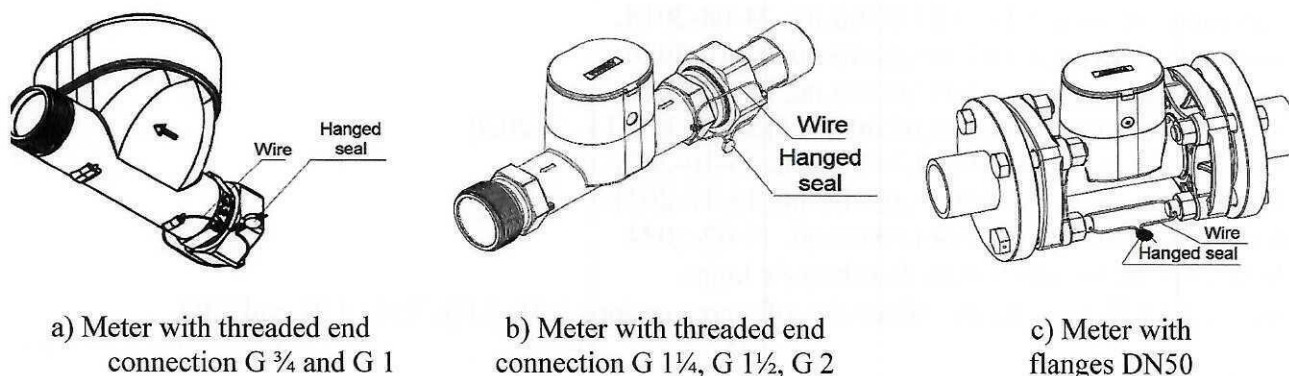
Fig. 5. Sealing of the water meter QALCOSONIC W1 after installation
