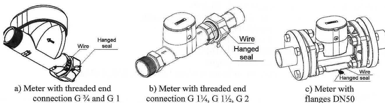
Fig. 5. Sealing of the water meter QALCASONIC W1 after installation
