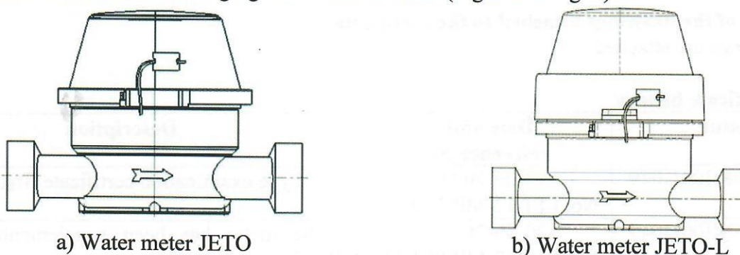
Fig. 3. Sealing of the water meter JETO and JETO-L
