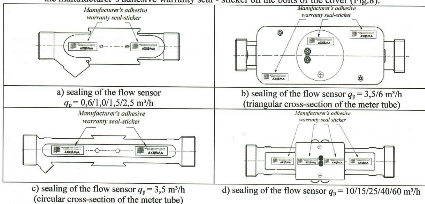
Fig.8. Sealing of the flow sensor
