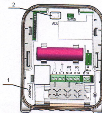
Fig. 5. Additional sealing of the combined device calculator
