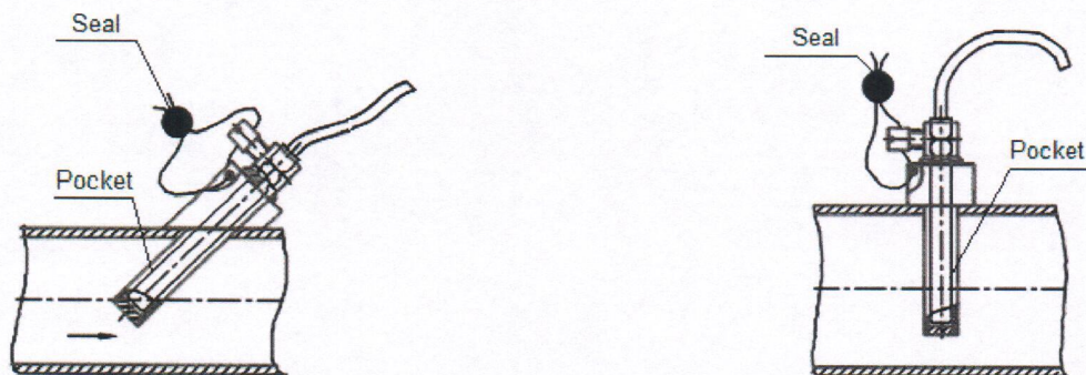
Fig. 7. Sealing of the PL type temperature probes
