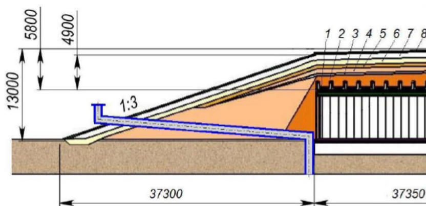
Figure 2. Composition (cross-section) of the 5.8 m thick engineered barrier after transformation of the storage facility (bld. 158) into a repository: (1) drainage layer; (2) insulating clay layer; (3) drainage layer; (4) protective clay layer; (5–7) drainage layers; (8) vegetation layer)
