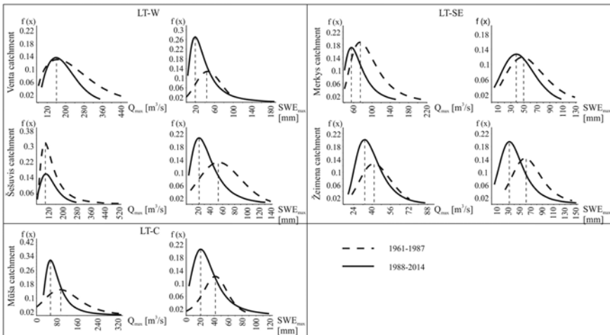
Fig. 3.6. Probability distributions of Q_{max} and SWE_{max} in the rivers of Venta, Šešuvis, Mūša, Merkys and Žeimena according to best fit distributions in the periods of 1961-1987 and 1988-2014
