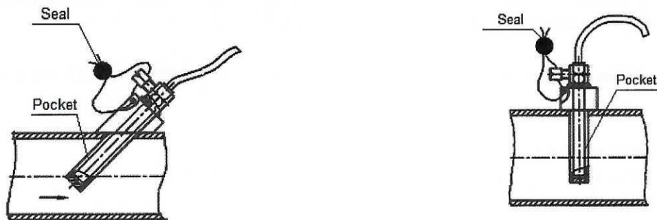
Fig. 9. Sealing of the PL type temperature probes
