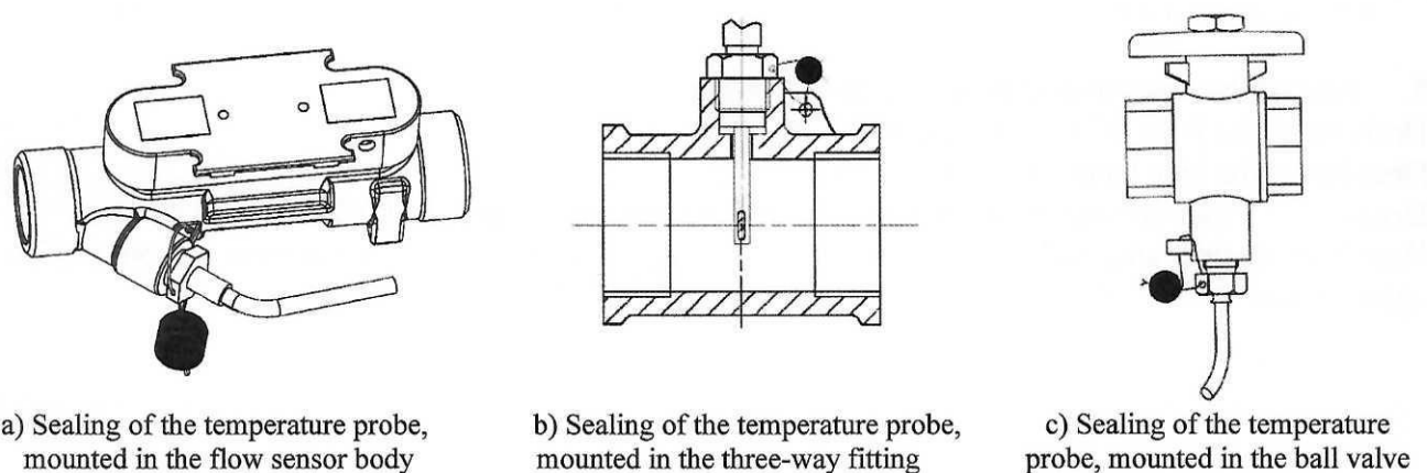
Fig. 10. Sealing of the DS type temperature probes
