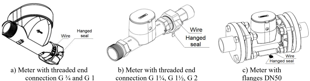
Fig. 5. Sealing of the water meter QALCOSONIC W1 after installation
