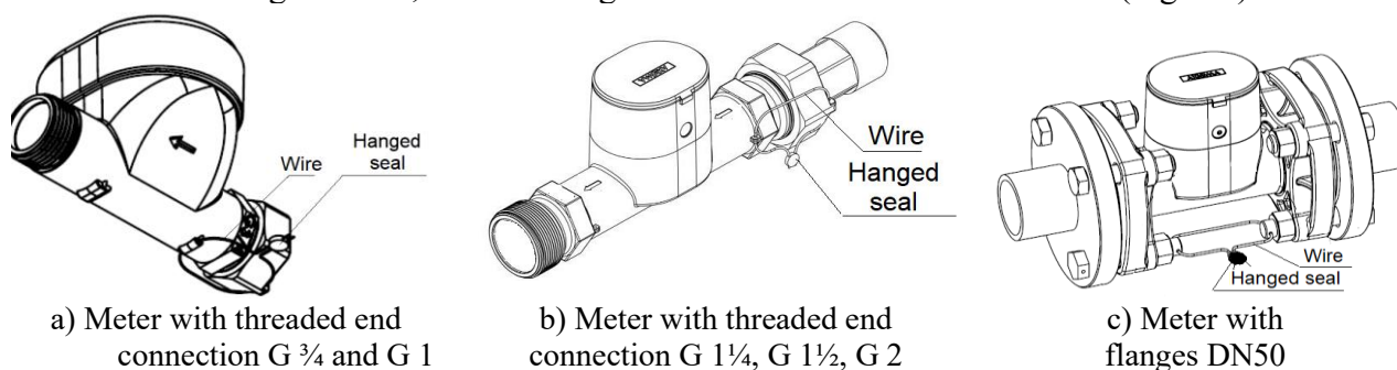
Fig. 5. Sealing of the water meter QALCASONIC W1 after installation
