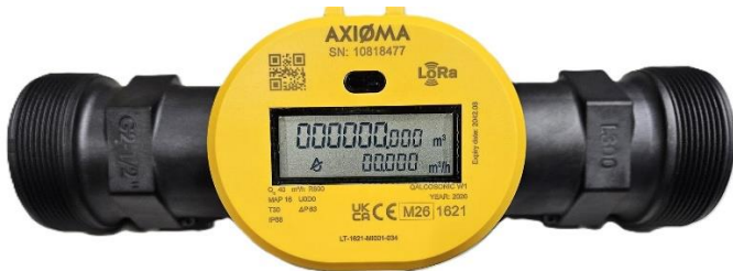
Fig. 6. Water meter QALCASONIC W1, Q_3 = 16/25/40 \text{ m}^3 , with threaded end connection G 2 1/2
