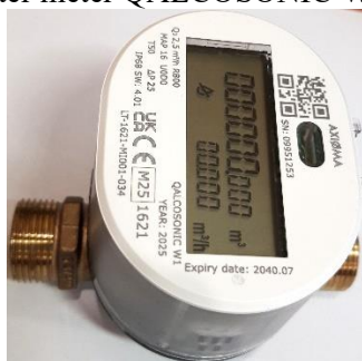
Fig.2. Water meter QALCASONIC W1, Q_3 = 1,6/2,5 \text{ m}^3 , G \frac{3}{4} , with brass body
