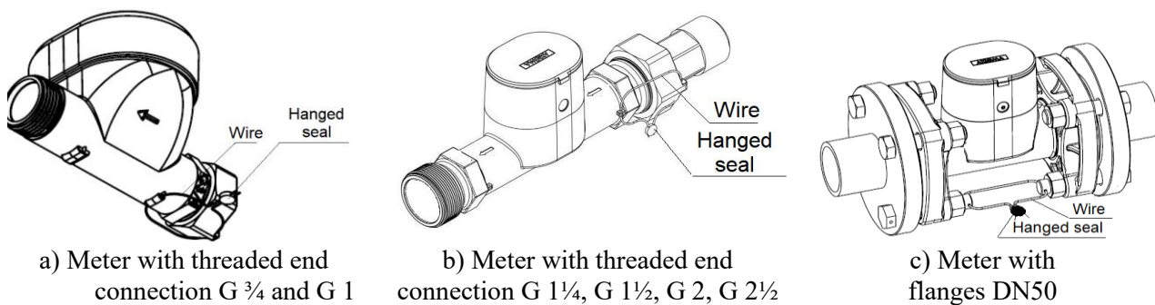
Fig. 8. Sealing of the water meter QALCOSONIC W1 after installation
